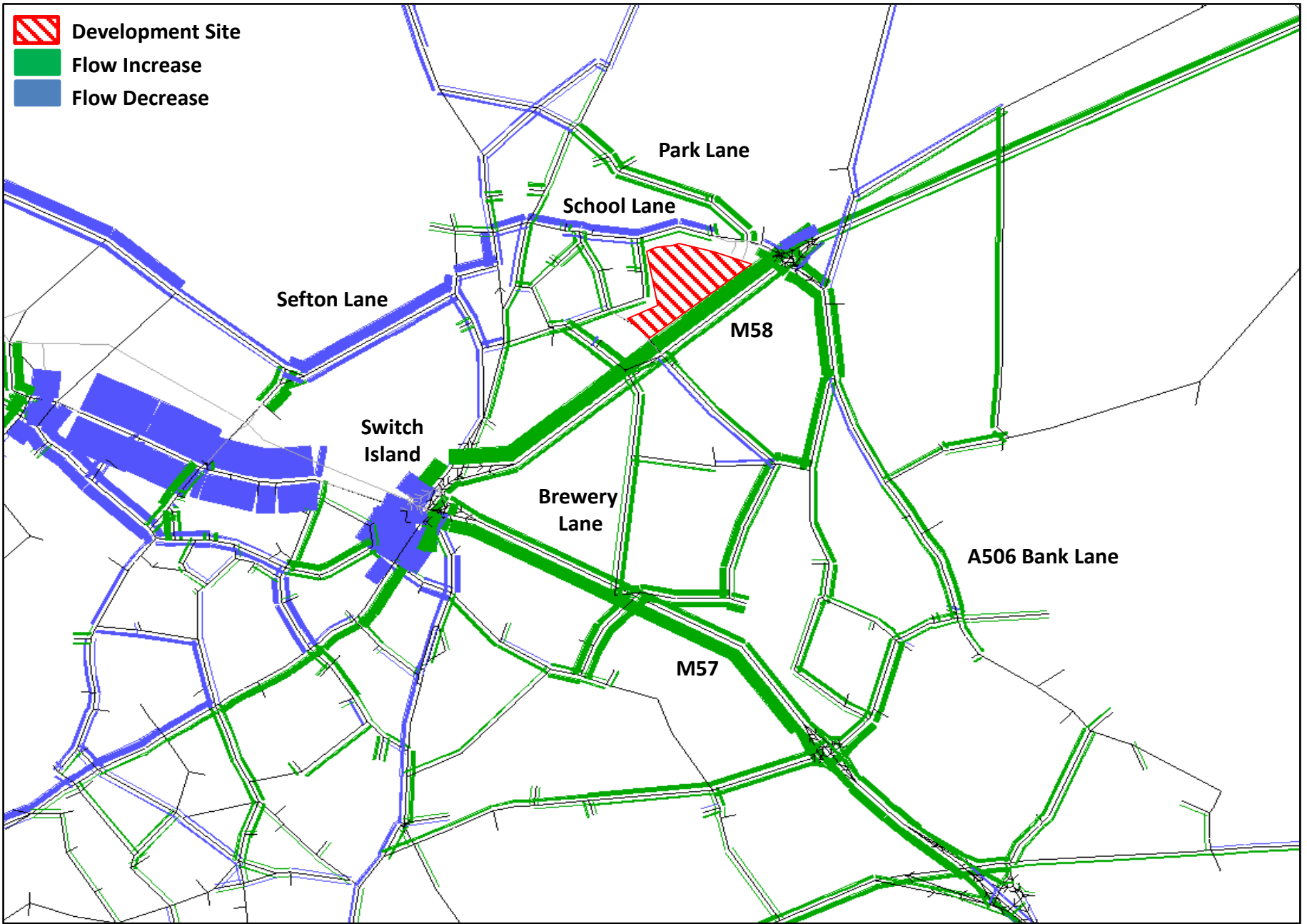
2024 Flow Comparison (AM): Do Something minus Base – Without slips, without spine
