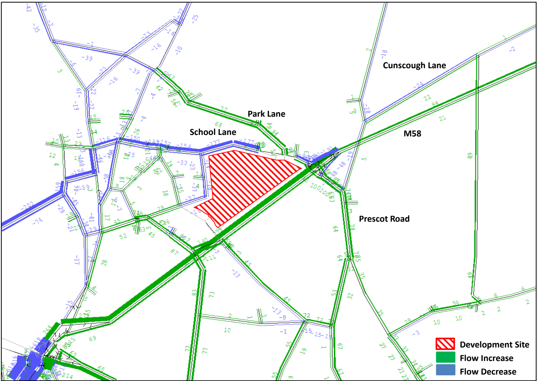
2024 Flow Comparison (AM): Do Something minus Base – Without slips, Including spine – Site zoom
