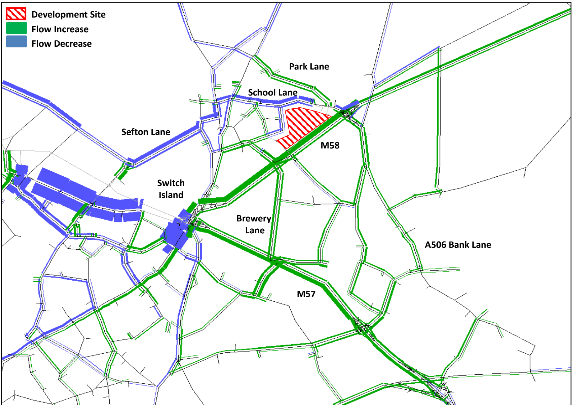
2024 Flow Comparison (AM): Do Something minus Base – Without slips, Including spine
