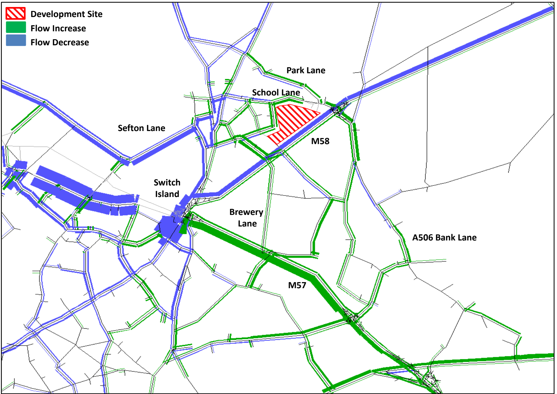
2024 Flow Comparison (PM): Do Something minus Base – Without slips, without spine
