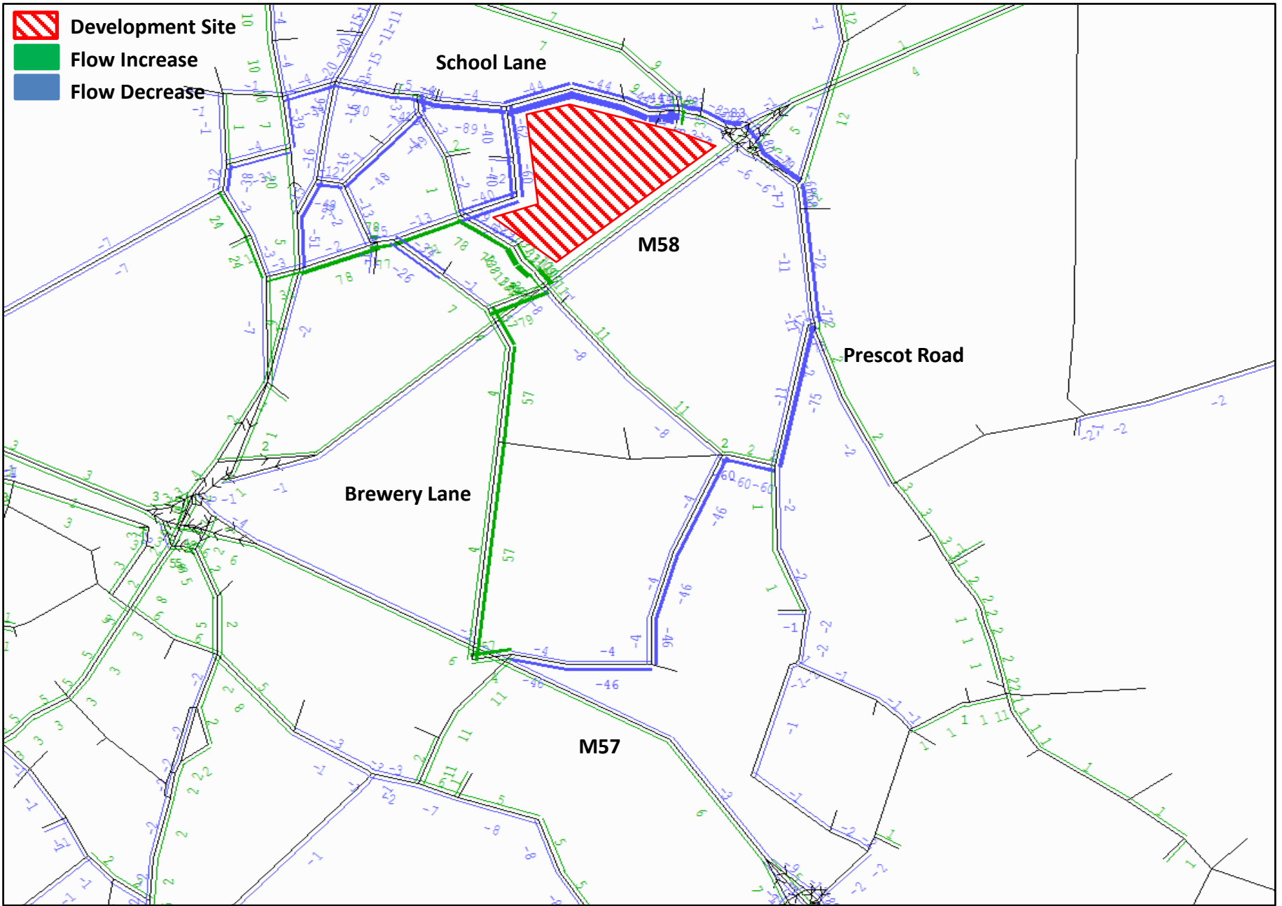
2024 Flow Comparison (PM): Including Spine minus Without Spine (Without Slips)
