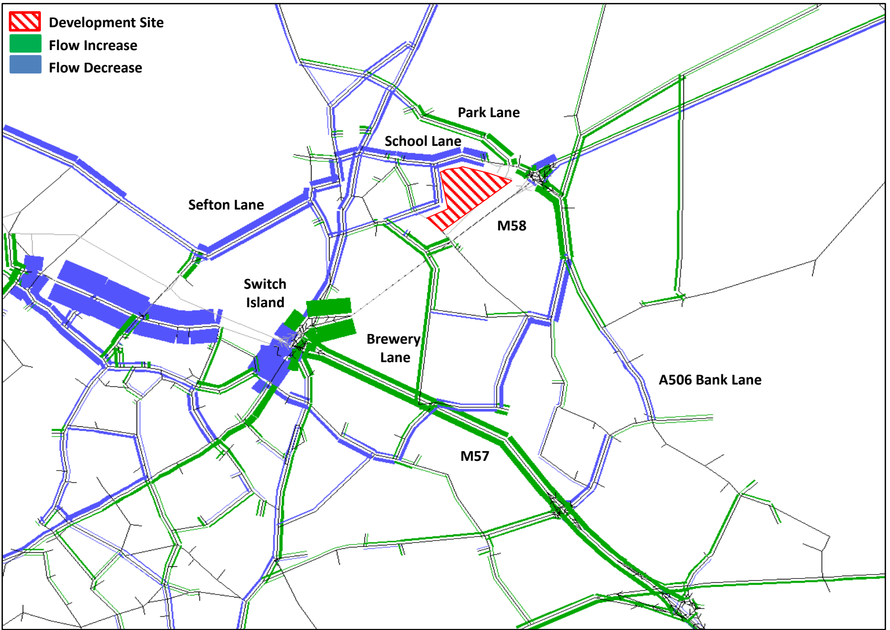
2024 Flow Comparison (AM): Do Something minus Base – Including slips, including spine
