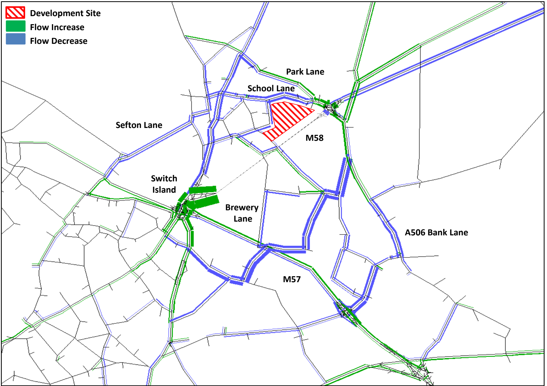
2024 Flow Comparison (AM): Including Slips minus Without Slips (Without Spine)
