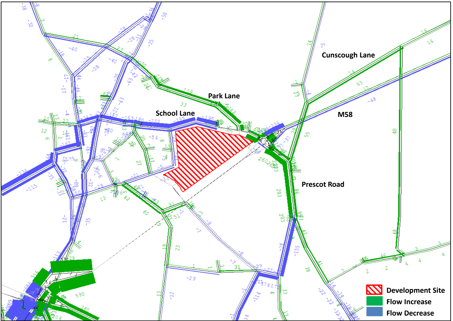
2024 Flow Comparison (AM): Do Something minus Base – Including slips, without spine – Site zoom
