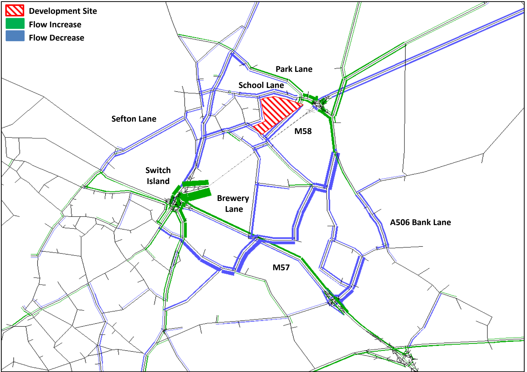
2024 Flow Comparison (AM): Including Slips minus Without Slips (Including Spine)
